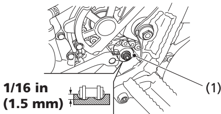
(1) chain roller
