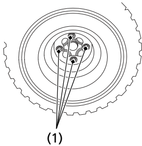
(1) wheel nuts
