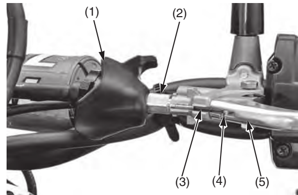
(1) dust cover (2) adjuster (3) clutch cable (4) clutch cable end (5) clutch lever
