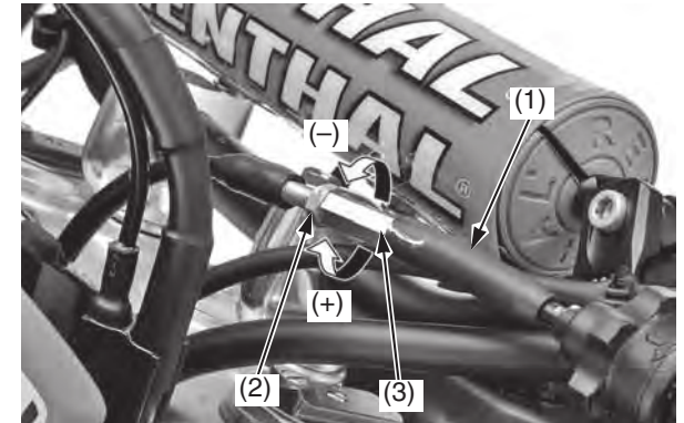
(1) dust cover (2) lock nut (3) integral cable adjuster (+) increase freeplay (–) decrease freeplay
