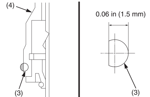
(3) wear ring
