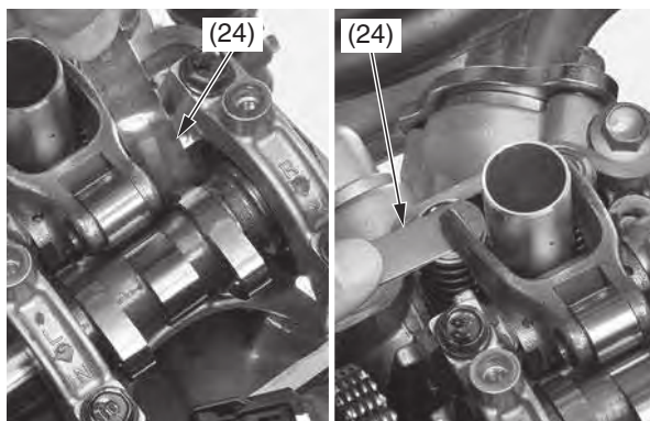
(24) feeler gauge
