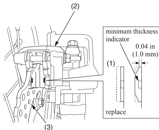
(1) brake pads (2) rear brake caliper (3) brake disc
