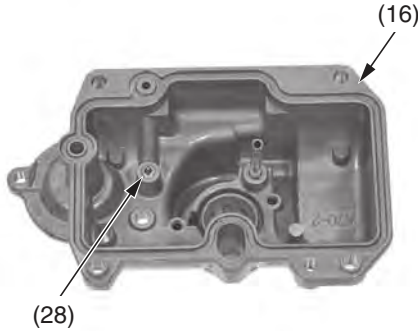
(16) float bowl (28) leak jet
