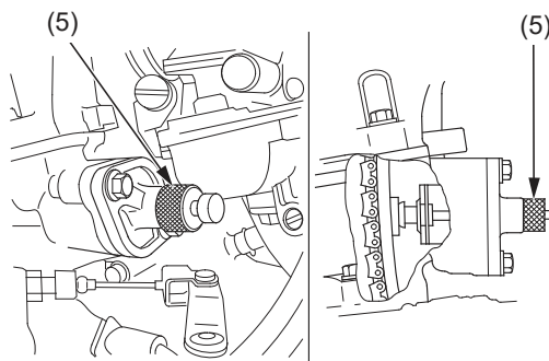
(5) tensioner stopper
