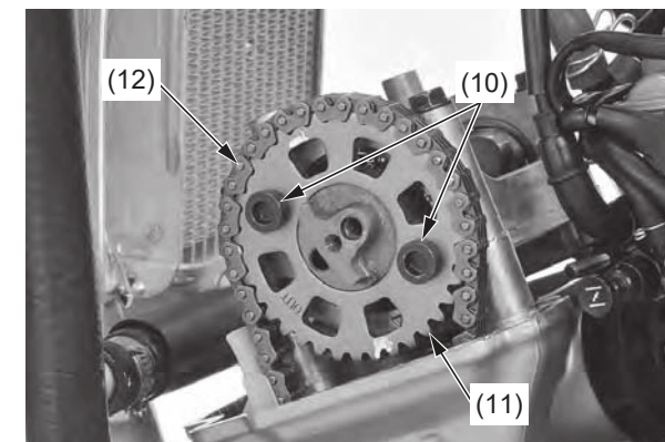
(10) cam sprocket bolts (12) cam chain (11) cam sprocket
