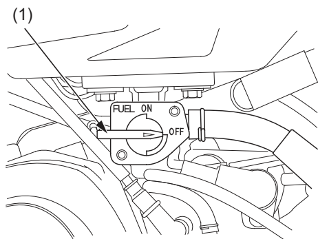
(1) fuel valve
