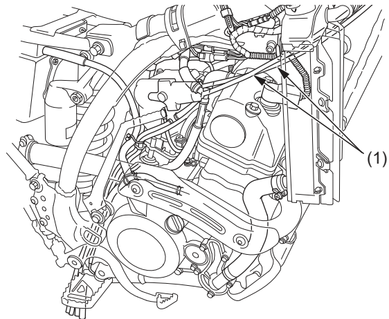
(1) throttle cables
