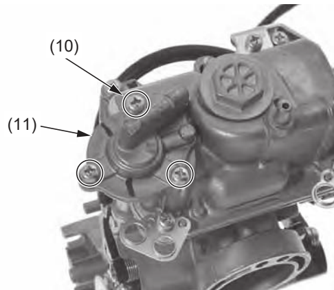
(10) accelerator pump cover screws (11) accelerator pump cover
