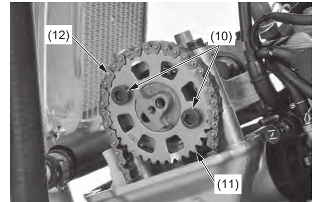
(10) cam sprocket bolts (11) cam sprocket (12) cam chain
