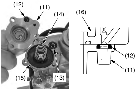
(11) accelerator pump cover (12) U-ring (13) O-ring (14) spring (15) diaphragm (16) float bowl
