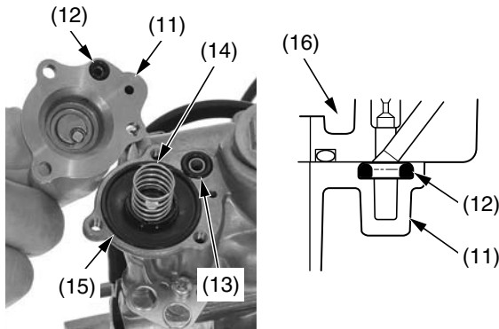
(11) accelerator pump cover (12) U-ring (13) O-ring
