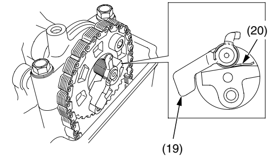
(19) decompressor weight (20) return spring
