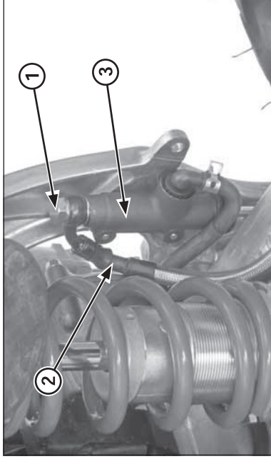
(1) OIL BOLT (2) BRAKE HOSE (3) MASTER CYLINDER
