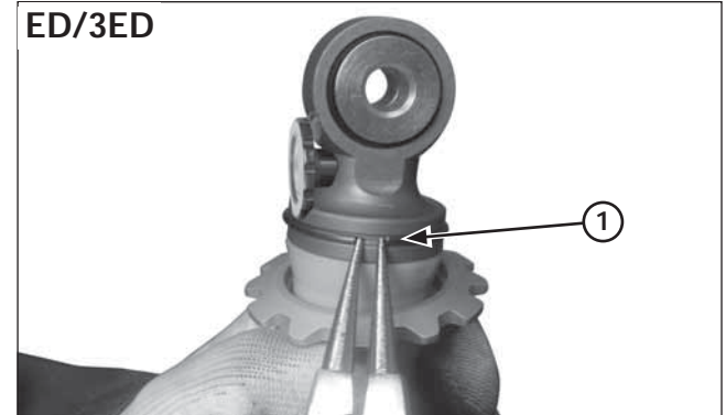
(1) SEEGER
