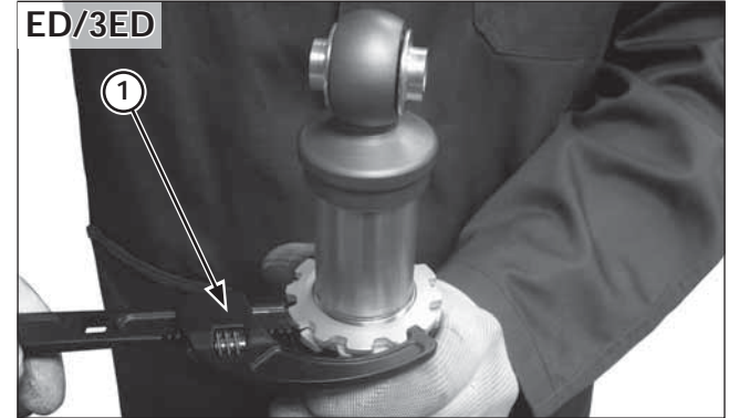
(1) SPANNER WRENCH
