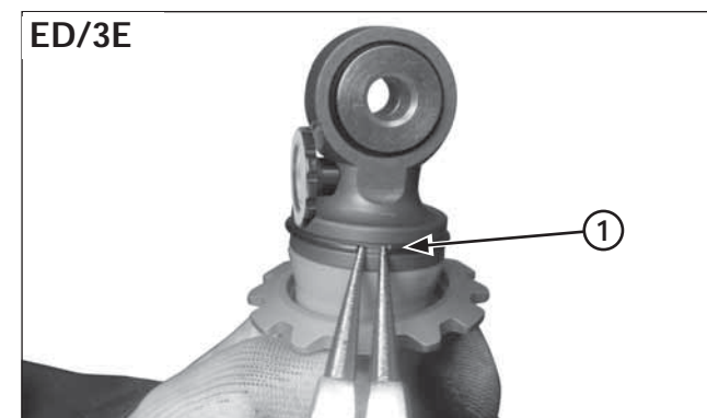
(1) CIRCLIP
