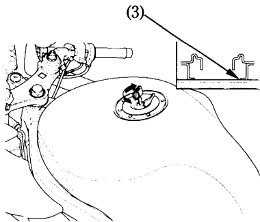
(3) Filler neck
