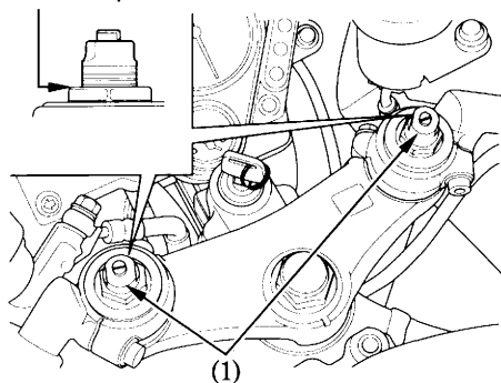
(1) Preload adjuster
