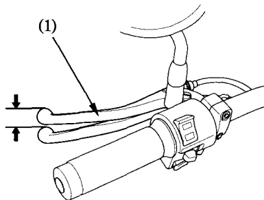
(1) Clutch lever
