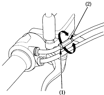
(1) Lock nut
