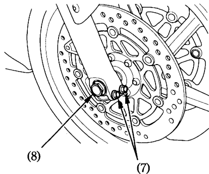
(7) Axle pinch bolts
