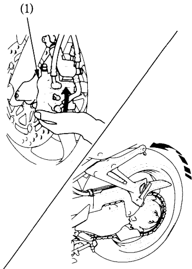
(1) Left caliper assembly
