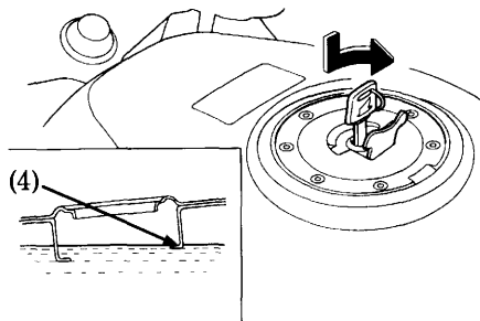
(4) Filler neck
