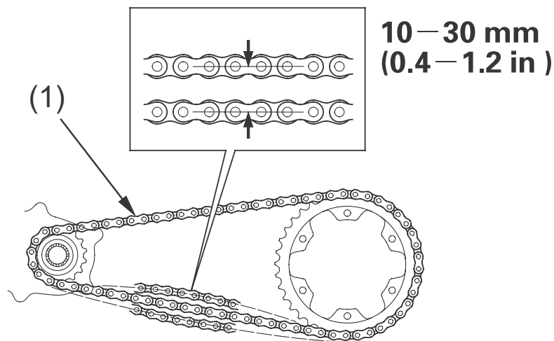
(1) drive chain
