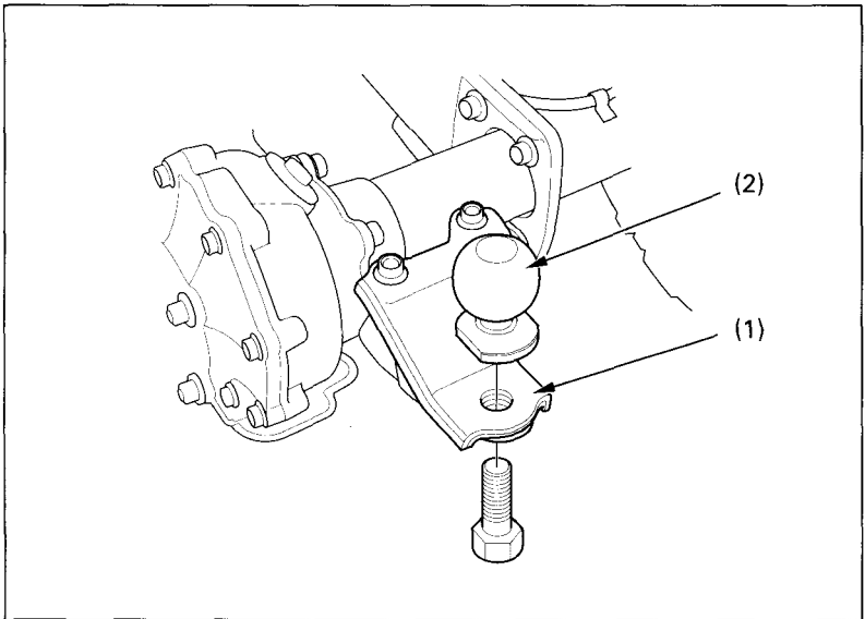
Fig. 2-34 (1) Trailer hitch
