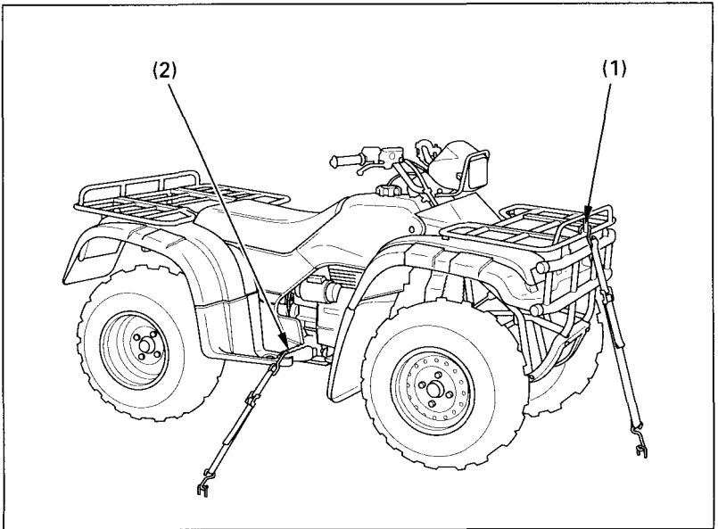
Fig. 4-40 Points to secure FOURTRAX with tie downs
