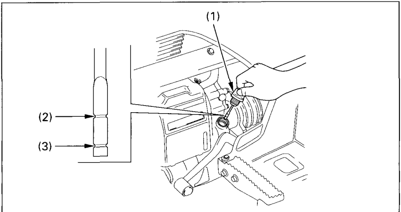
Fig. 4-10 (1) Oil filler cap/dipstick (2) Upper level mark (3) Lower level mark
