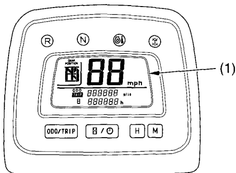
(1) multi-function display
