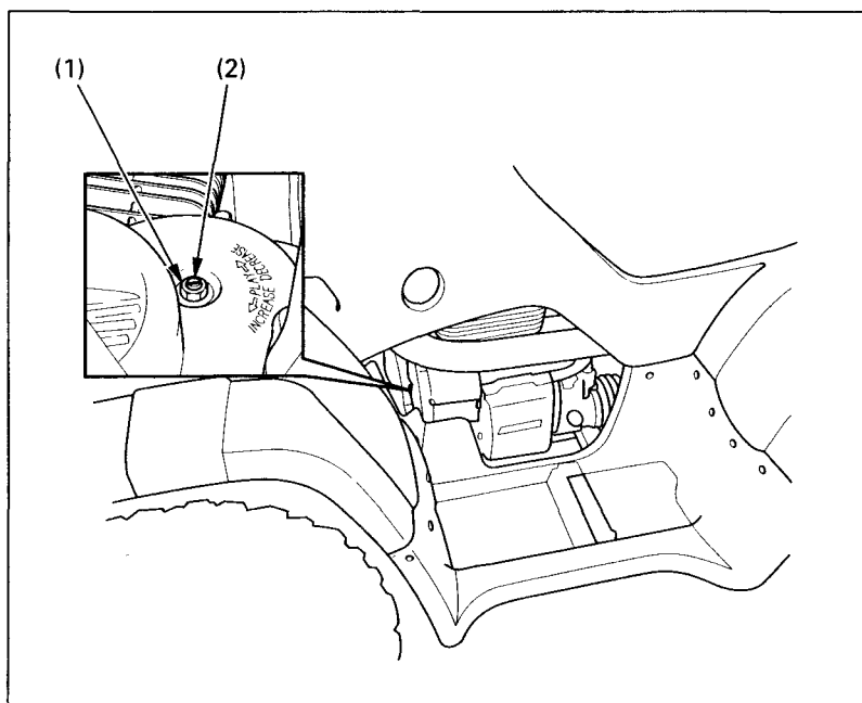
Fig. 4-17 (1) Lock nut
