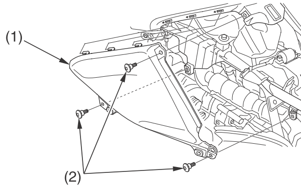
(1) left tank side cover
