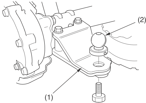
(1) trailer hitch
