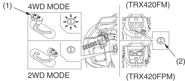
(1) 2WD/4WD select lever (2) 4WD indicator
