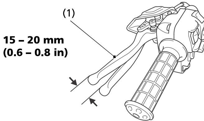
(1) rear brake lever/parking brake lever
