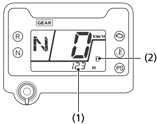
(2) hourmeter mark
