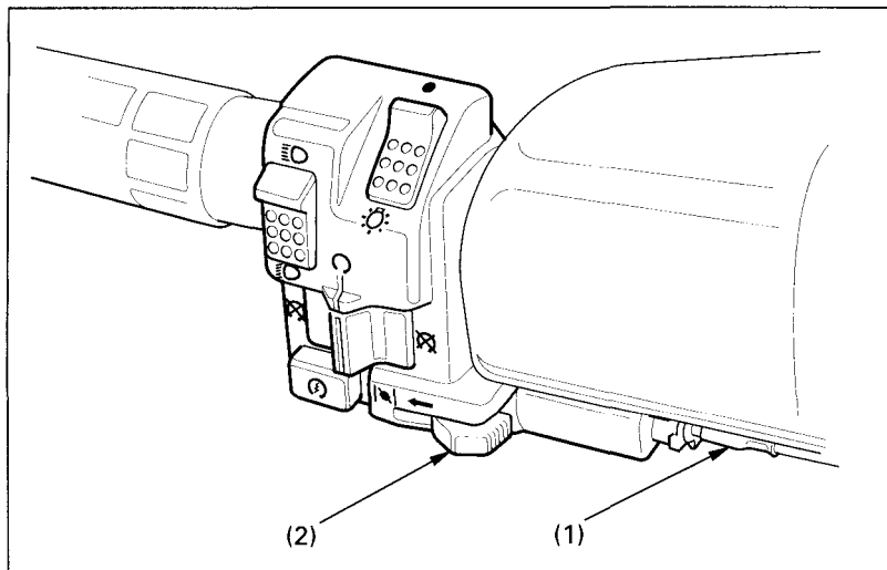
(2) Choke lever
