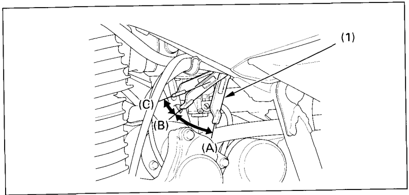
Fig. 3-9 (1) Choke lever
