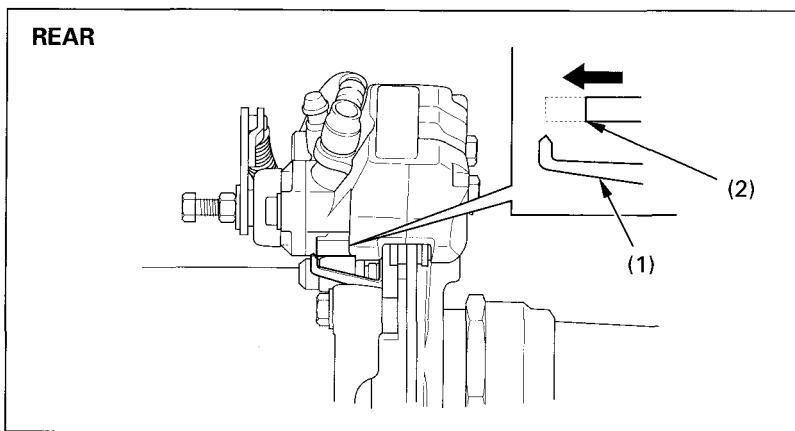
Fig. 4-26 (1) Wear indicator (2) Edge of reference mark
