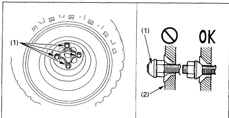
Fig. 4-30 (1) Wheel nuts
