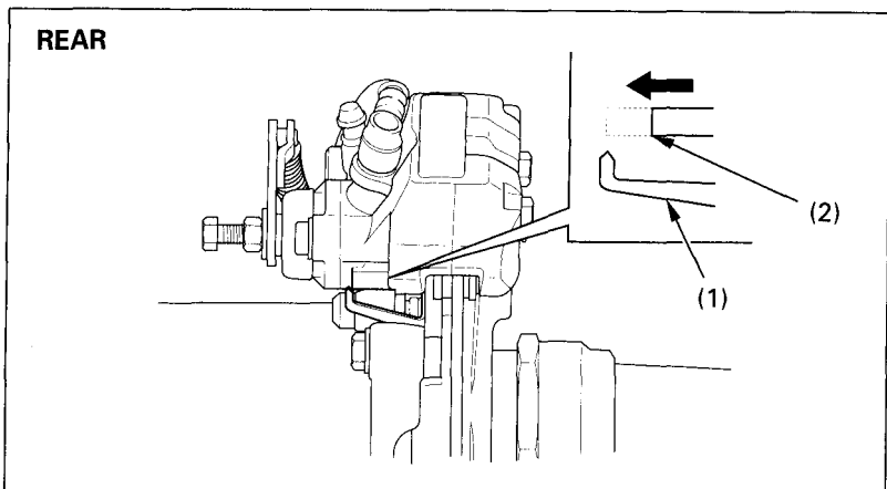
Fig. 4-27 (1) Wear indicator (2) Edge of reference mark
