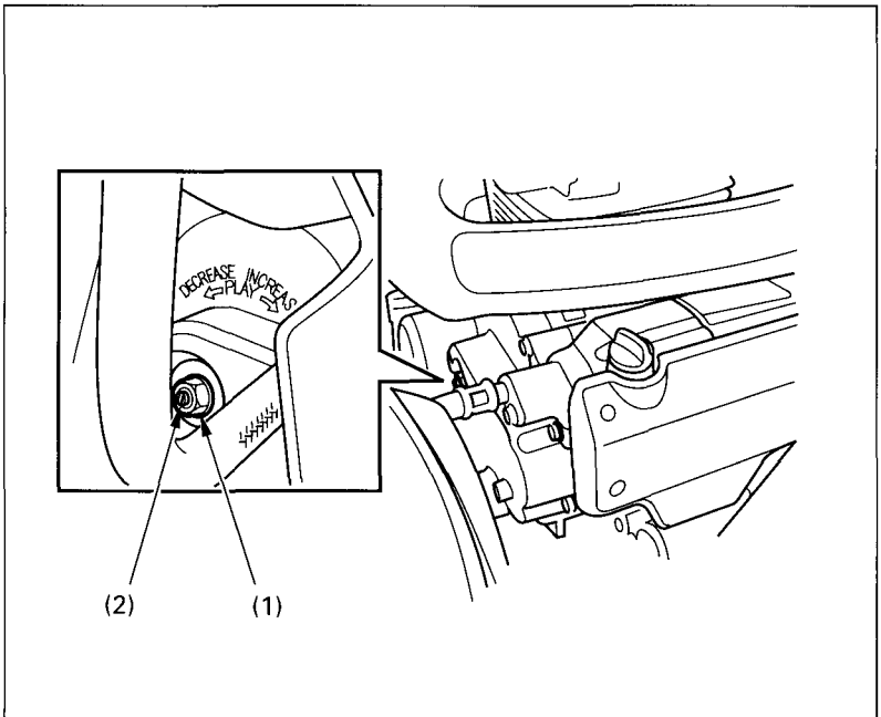
Fig. 4-15 (1) Lock nut
