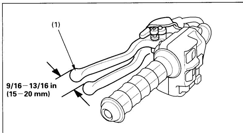
(1) Brake lever
