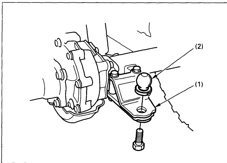
Fig. 2-31 (1) Trailer hitch
