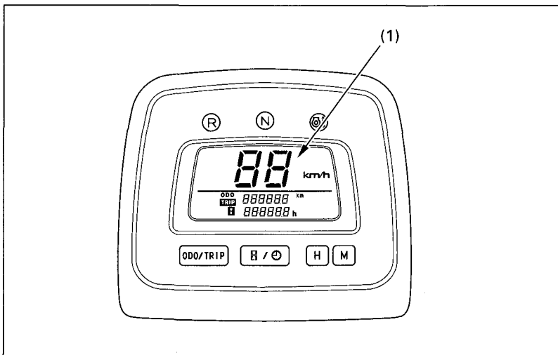
Fig. 2-15 (1) Multi-function display
