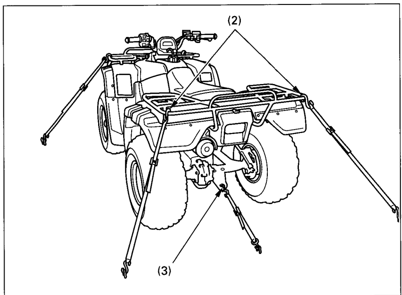
Fig. 4-42 Points to secure FOURTRAX with tie downs
