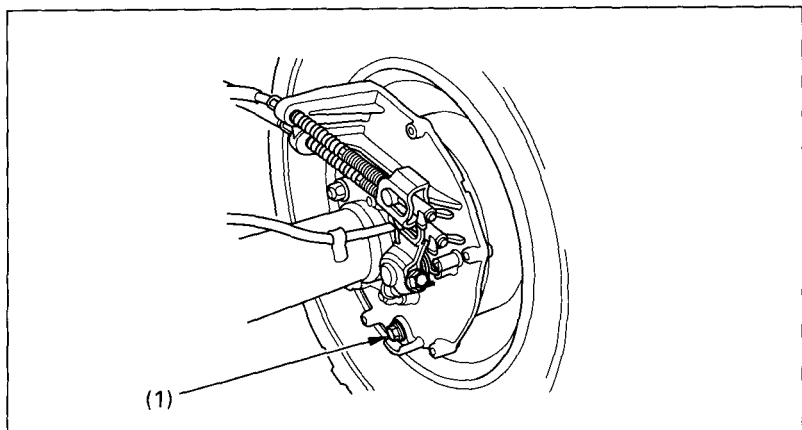
(1) Rear brake drain bolt
