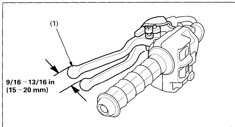
(1) Brake lever
