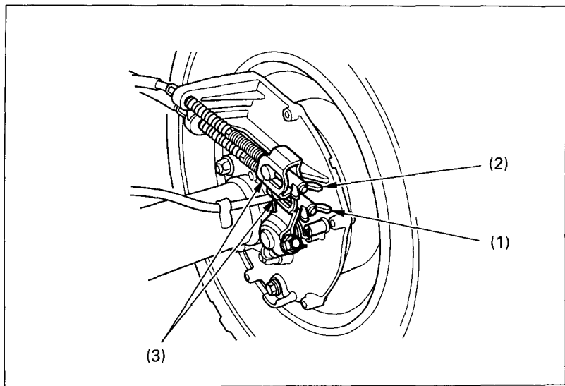
Fig. 4-30 (1) Brake pedal adjusting nut (2) Brake lever adjusting nut (3) Brake arm pin
